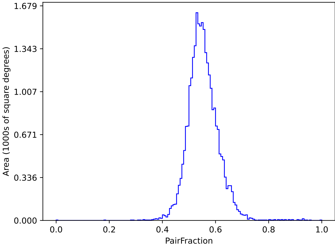
early_ss_template_fpextra3.0_v3.4_10yrs (g or r or i): PairFraction
