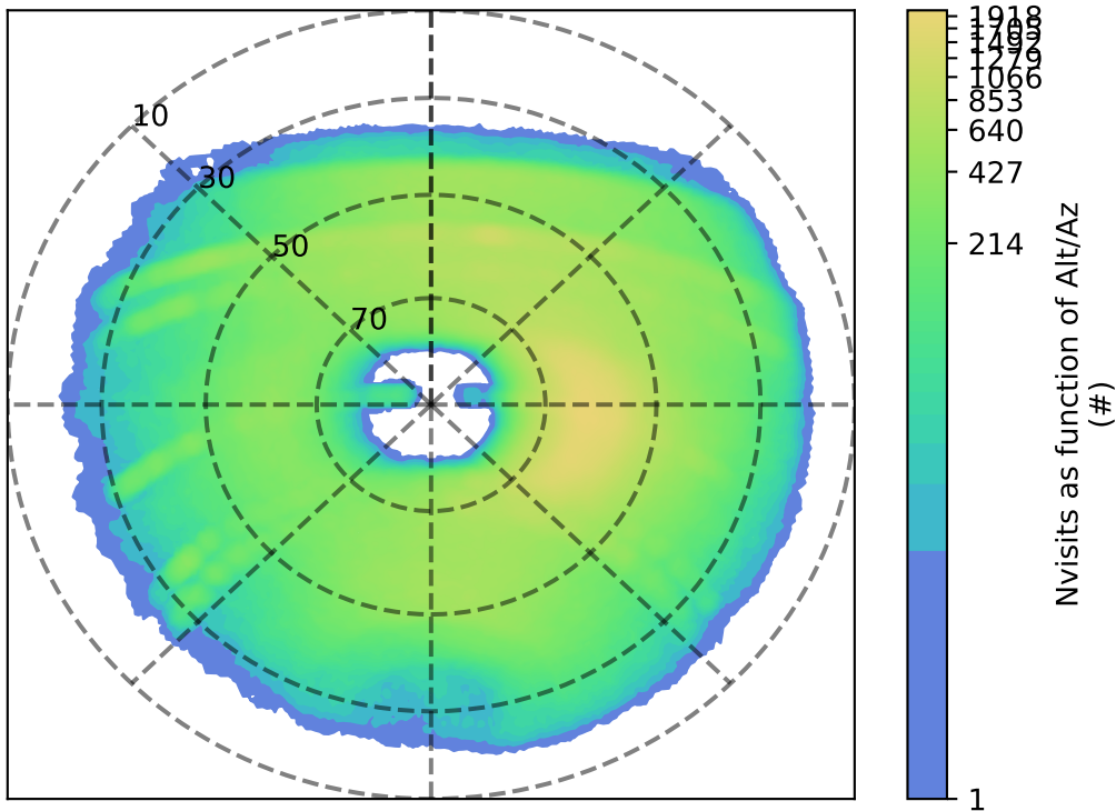
early_ss_template_fpextra3.0_v3.4_10yrs y: Nvisits as function of Alt/Az
