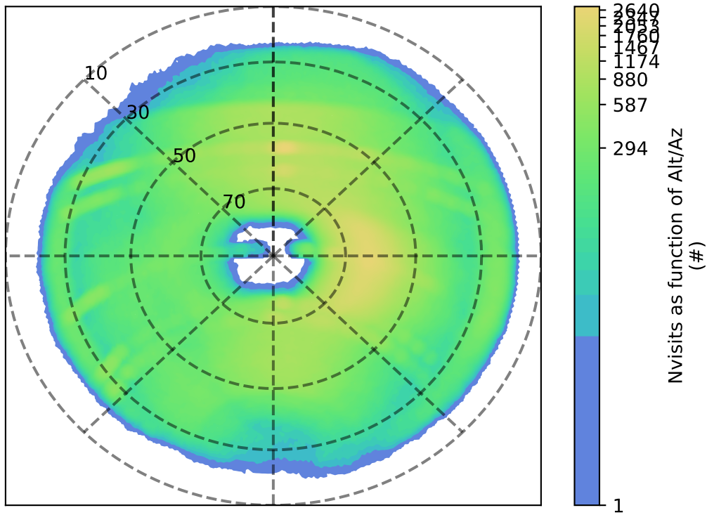
early_ss_template_fpextra3.0_v3.4_10yrs i: Nvisits as function of Alt/Az
