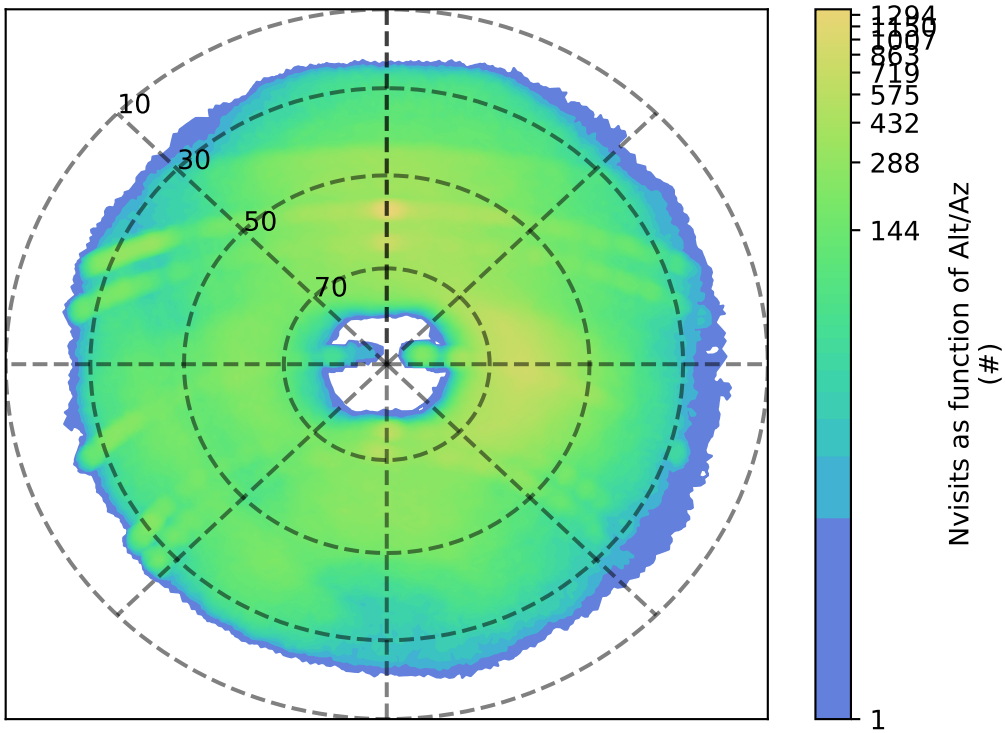
early_ss_template_fpextra3.0_v3.4_10yrs g: Nvisits as function of Alt/Az
