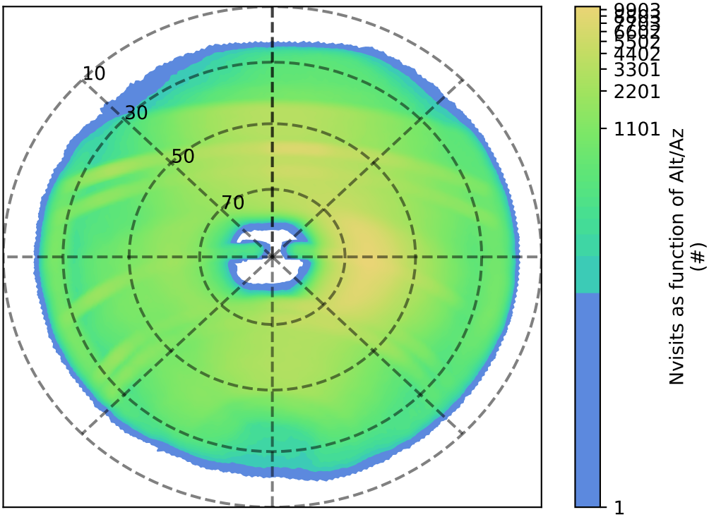
early_ss_template_fpextra3.0_v3.4_10yrs : Nvisits as function of Alt/Az
