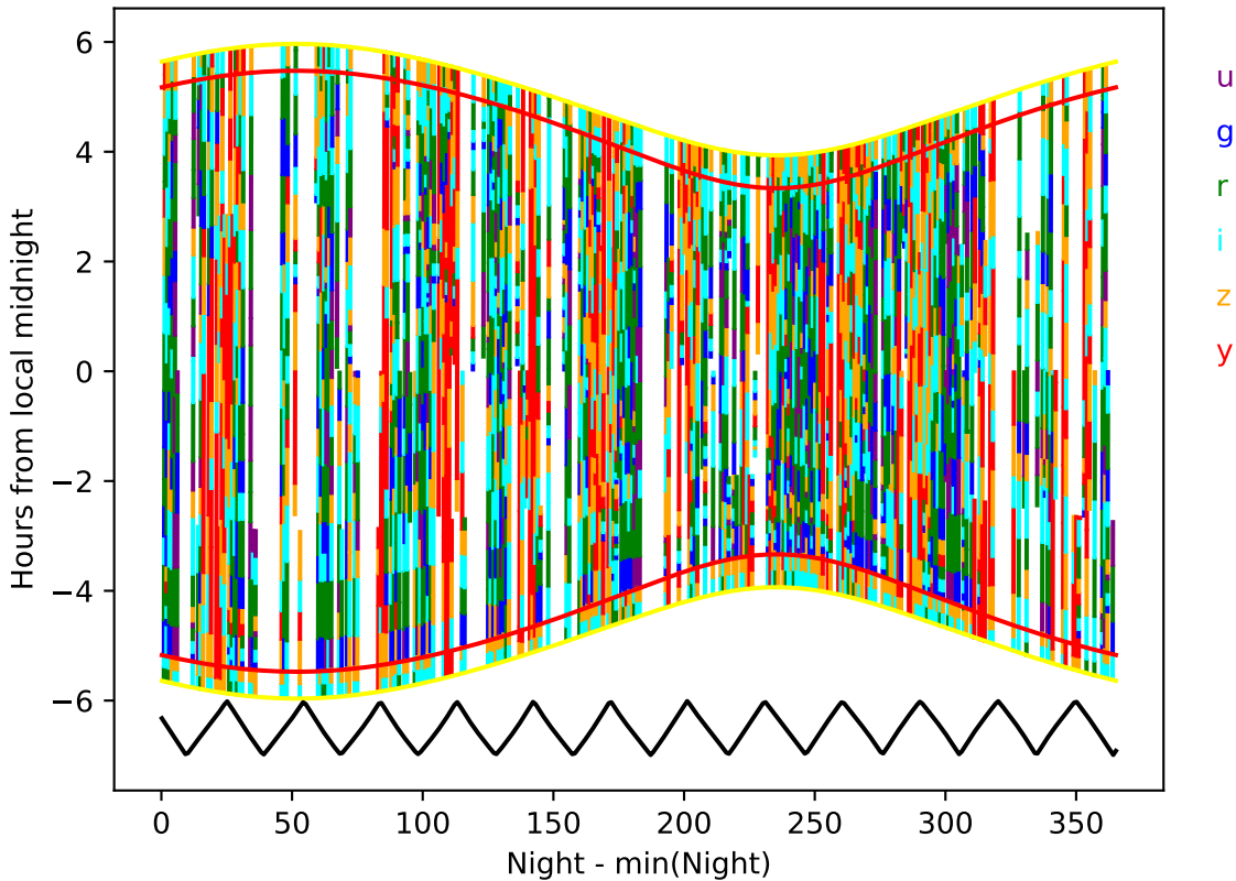
early_ss_template_fpextra3.0_v3.4_10yrs year 7-8: Hourglass
