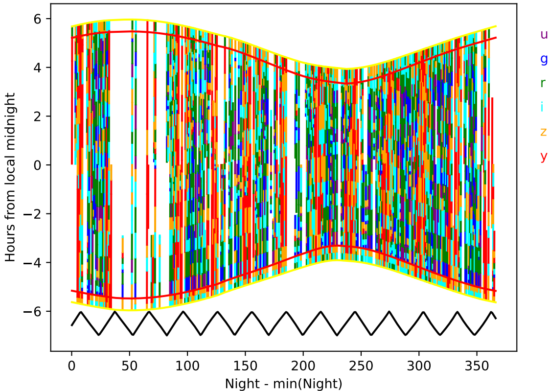
early_ss_template_fpextra3.0_v3.4_10yrs year 3-4: Hourglass
