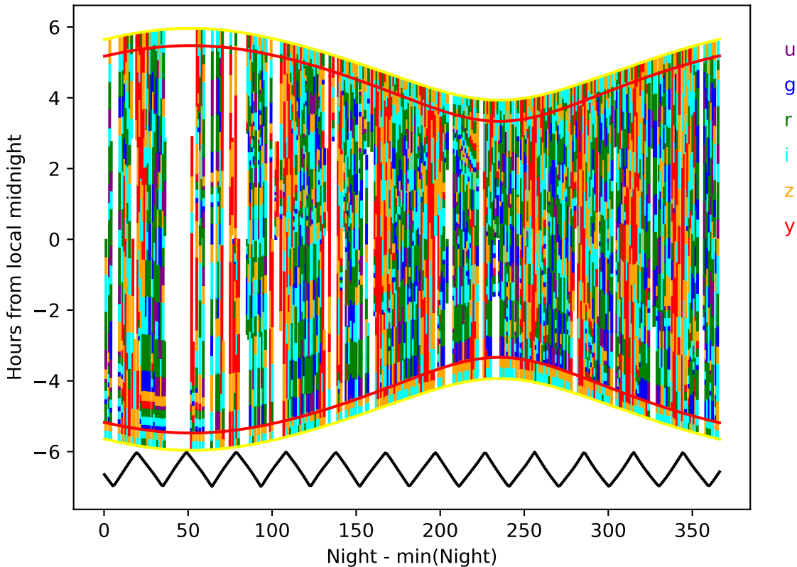
early_ss_template_fpextra3.0_v3.4_10yrs year 2-3: Hourglass
