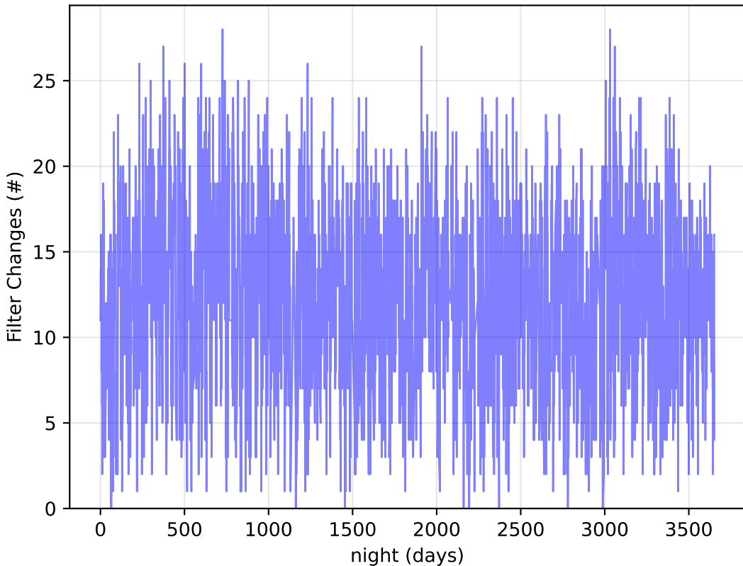
early_ss_template_fpextra3.0_v3.4_10yrs : Filter Changes
