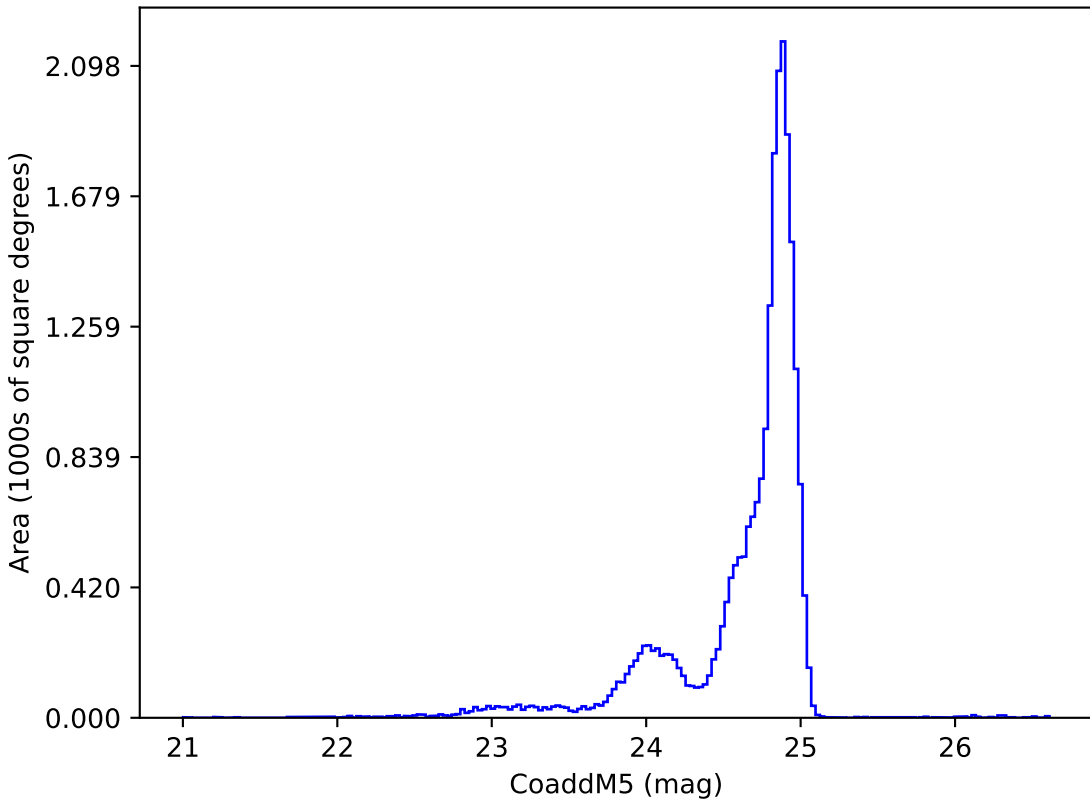
early_ss_template_fpextra3.0_v3.4_10yrs y: CoaddM5
