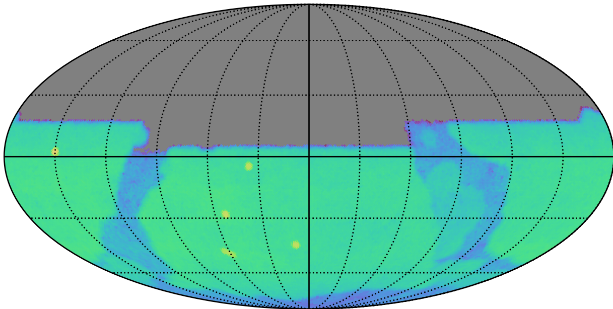
early_ss_template_fpextra3.0_v3.4_10yrs u: CoaddM5
