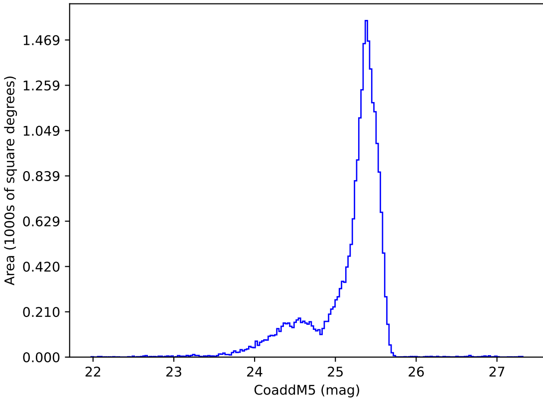
early_ss_template_fpextra3.0_v3.4_10yrs u: CoaddM5
