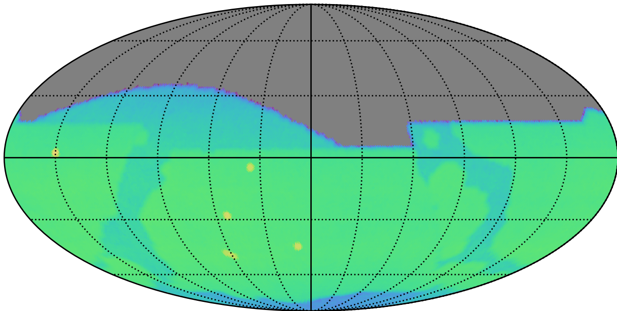
early_ss_template_fpextra3.0_v3.4_10yrs r: CoaddM5
