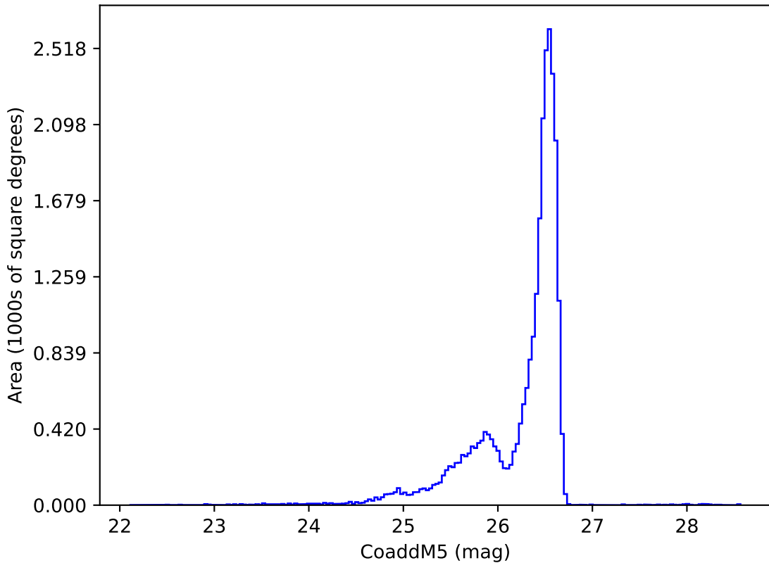
early_ss_template_fpextra3.0_v3.4_10yrs i: CoaddM5
