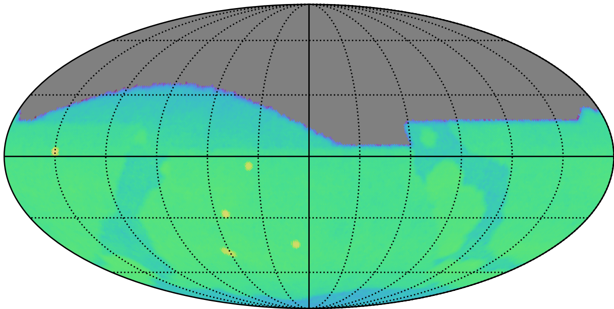
early_ss_template_fpextra3.0_v3.4_10yrs g: CoaddM5
