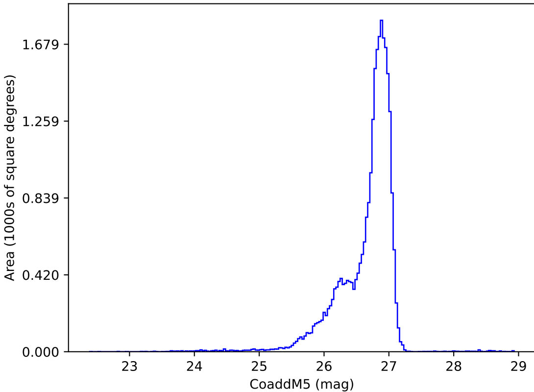
early_ss_template_fpextra3.0_v3.4_10yrs g: CoaddM5
