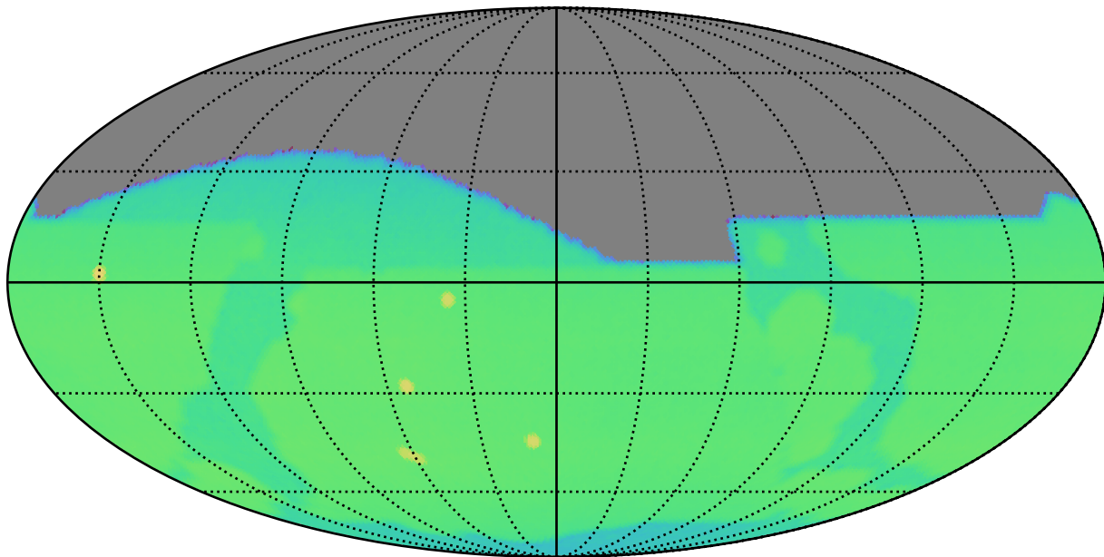
early_ss_template_fpextra3.0_v3.4_10yrs : CoaddM5
