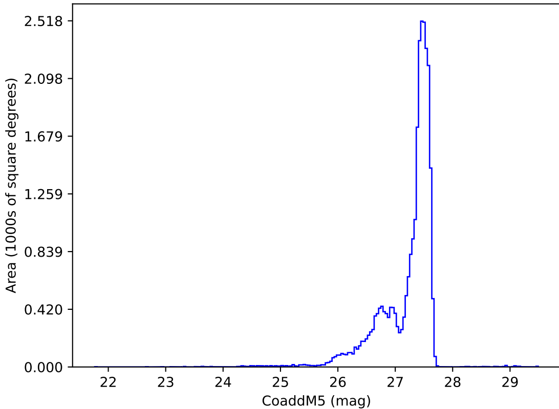
early_ss_template_fpextra3.0_v3.4_10yrs : CoaddM5
