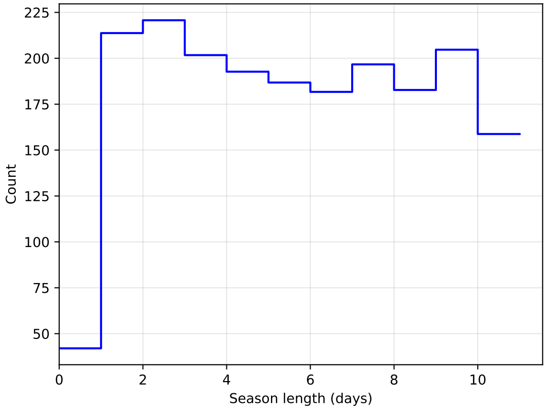
early_ss_template_fpextra3.0_v3.4_10yrs DD: COSMOS all bands: SeasonLength
