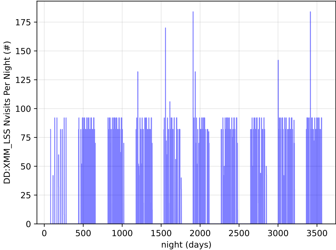
early_ss_template_fpextra3.0_v3.4_10yrs all bands: DD:XMM_LSS Nvisits Per Night
