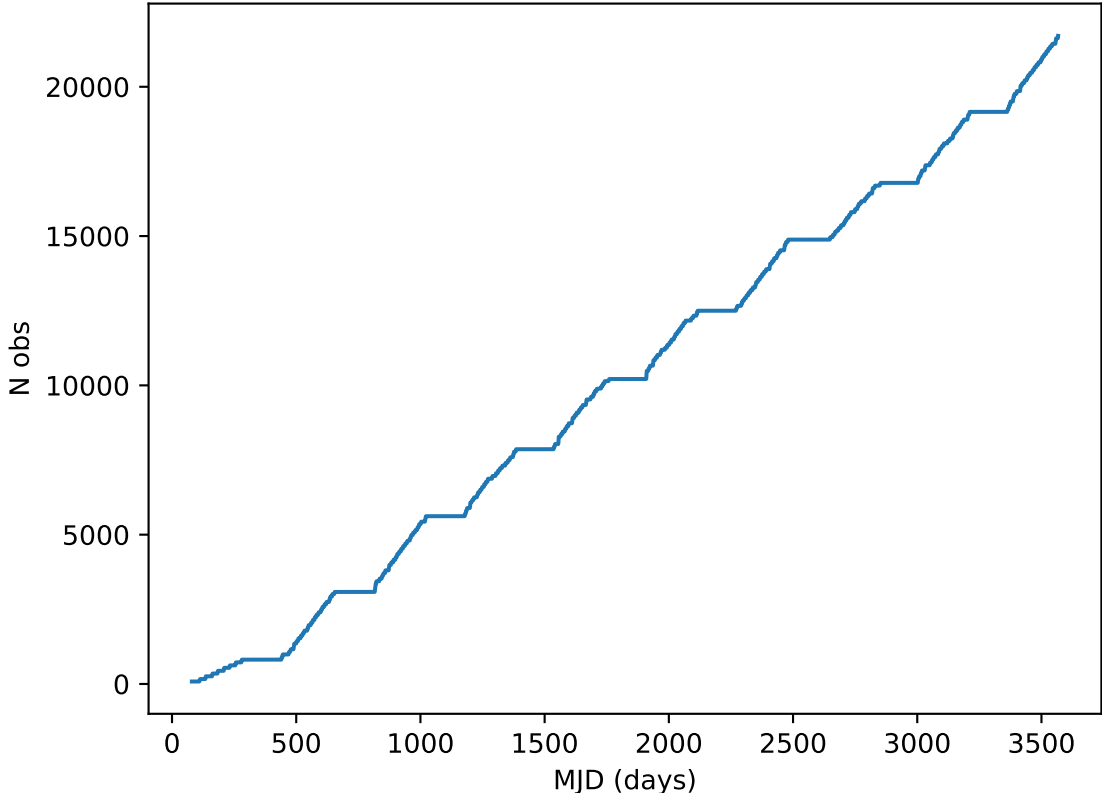
early_ss_template_fpextra3.0_v3.4_10yrs all bands: DD:XMM_LSS Cumulative NVisits
