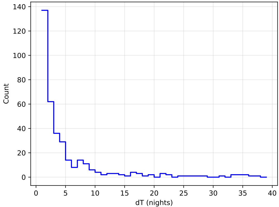
early_ss_template_fpextra3.0_v3.4_10yrs all bands: DD:WFD Delta Nights Histogram
