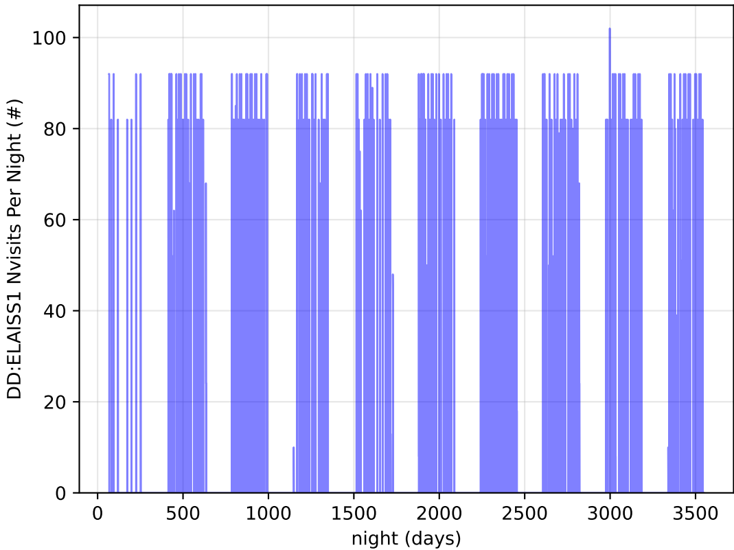
early_ss_template_fpextra3.0_v3.4_10yrs all bands: DD:ELAISS1 Nvisits Per Night
