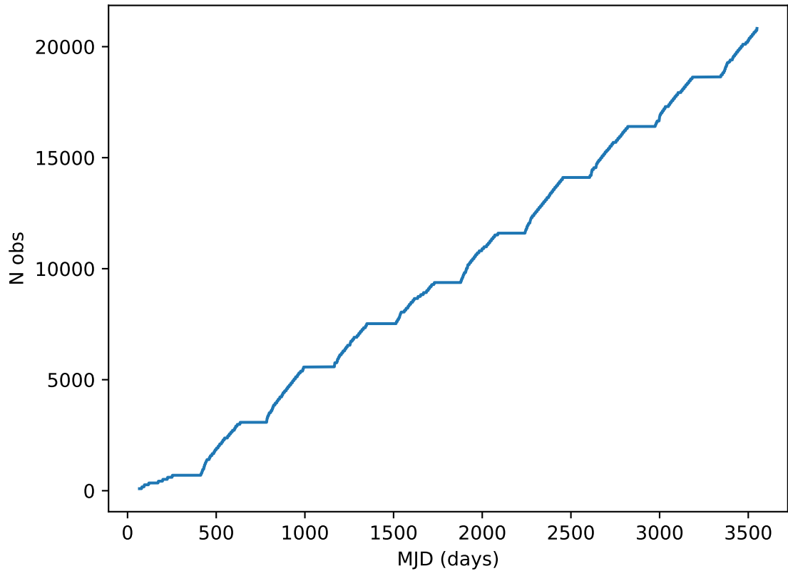
early_ss_template_fpextra3.0_v3.4_10yrs all bands: DD:ELAISS1 Cumulative NVisits
