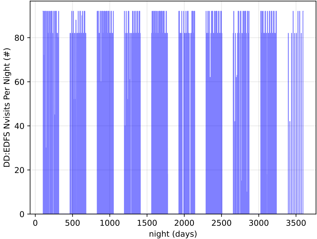
early_ss_template_fpextra3.0_v3.4_10yrs all bands: DD:EDFS Nvisits Per Night
