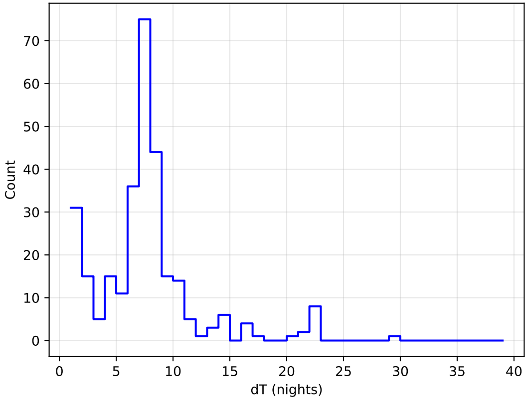
early_ss_template_fpextra3.0_v3.4_10yrs all bands: DD:EDFS Delta Nights Histogram
