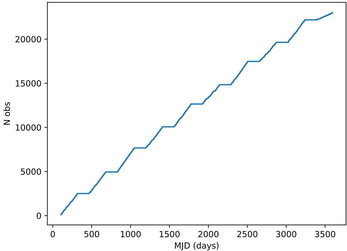
early_ss_template_fpextra3.0_v3.4_10yrs all bands: DD:EDFS Cumulative NVisits
