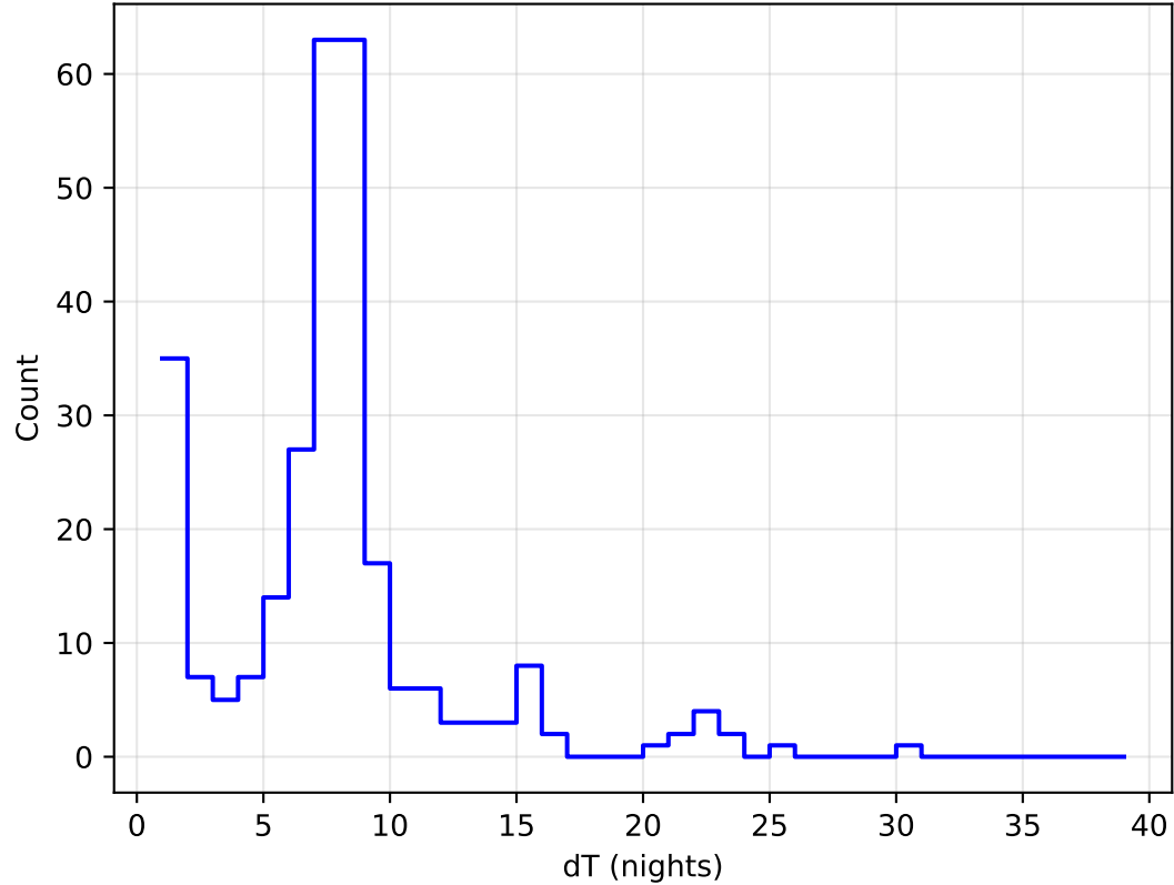
early_ss_template_fpextra3.0_v3.4_10yrs all bands: DD:ECDFS Delta Nights Histogram
