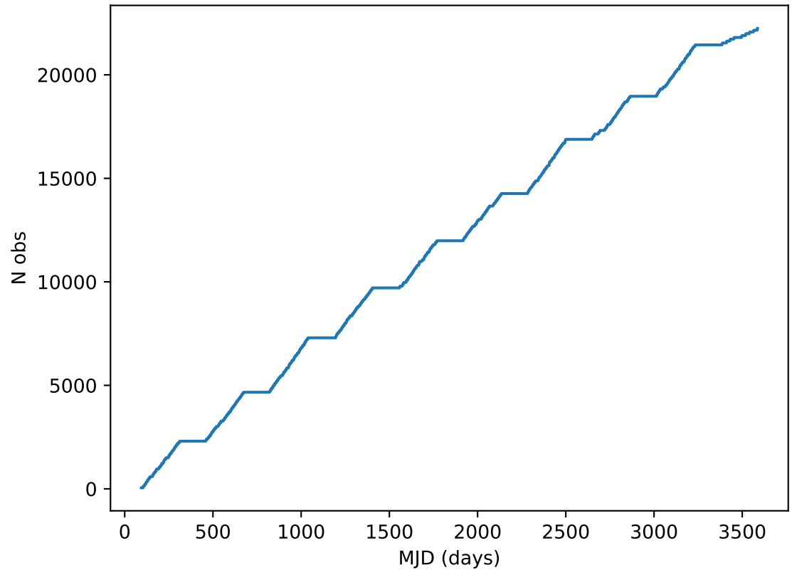
early_ss_template_fpextra3.0_v3.4_10yrs all bands: DD:ECDFS Cumulative NVisits
