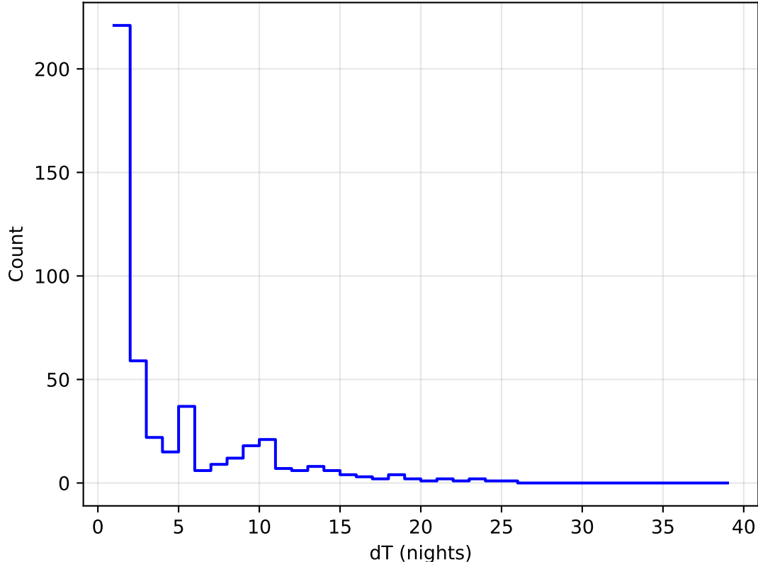
early_ss_template_fpextra3.0_v3.4_10yrs all bands: DD: COSMOS Delta Nights Histogram
