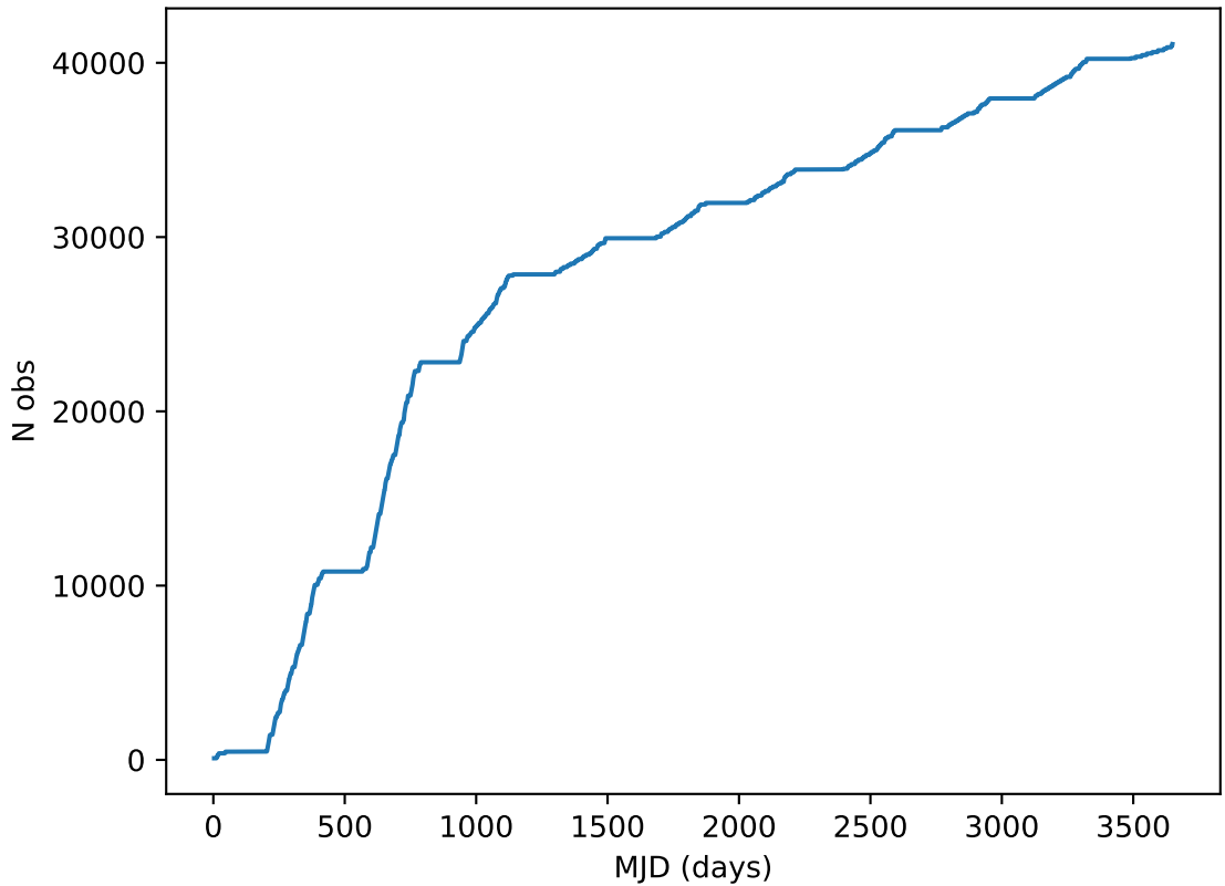
early_ss_template_fpextra3.0_v3.4_10yrs all bands: DD: COSMOS Cumulative NVisits
