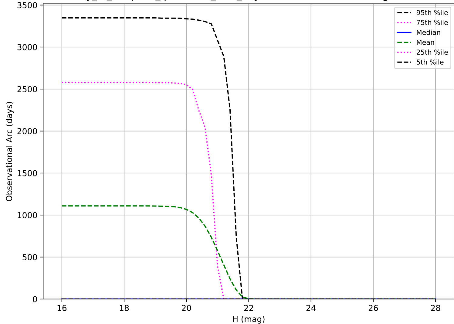
early_ss_template_fpextra2.0_v3.4_10yrs: Observational Arc Length Vatra
