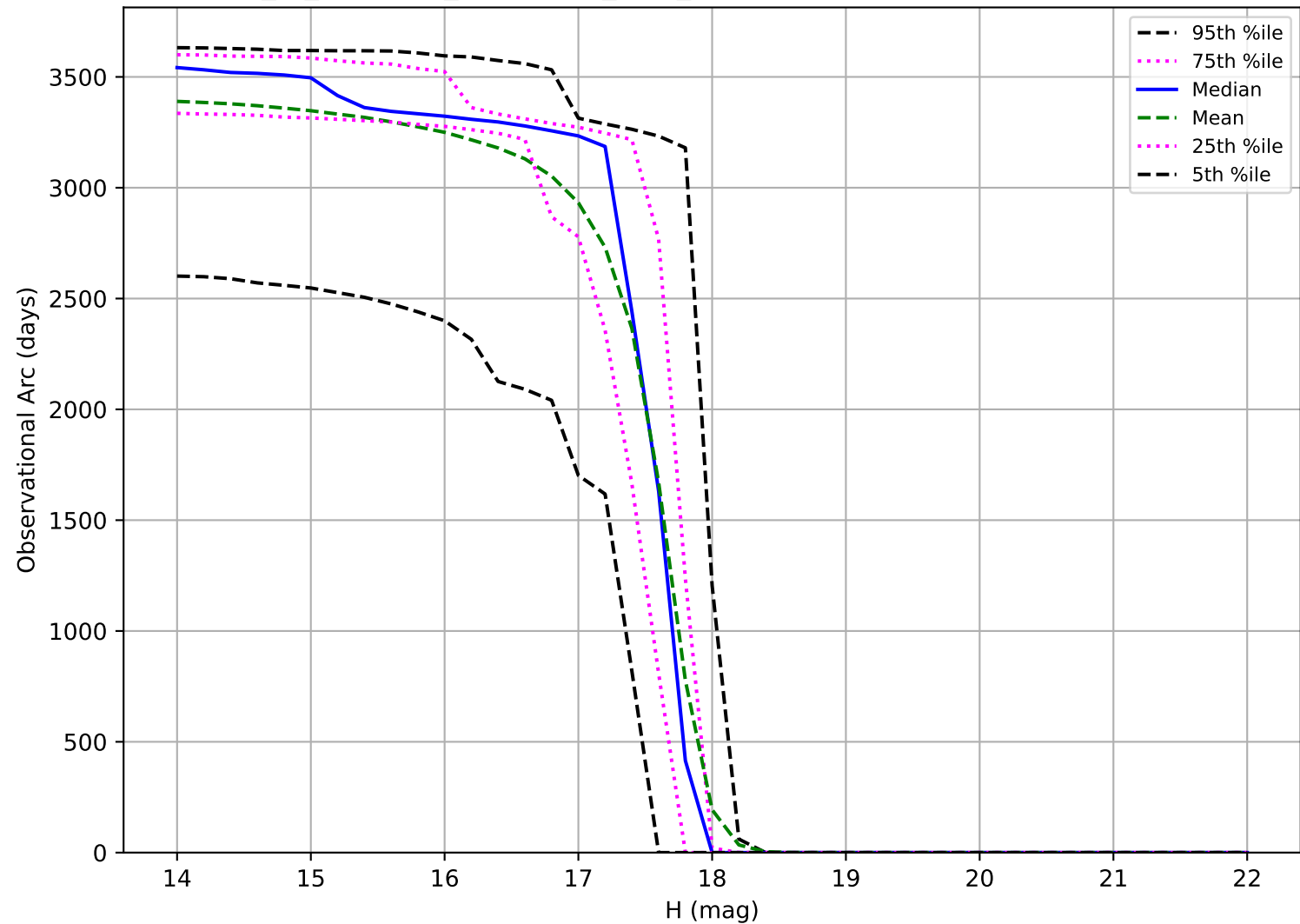
early_ss_template_fpextra2.0_v3.4_10yrs: Observational Arc Length Trojan
