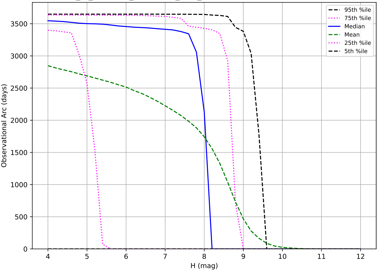
early_ss_template_fpextra2.0_v3.4_10yrs: Observational Arc Length TNO
