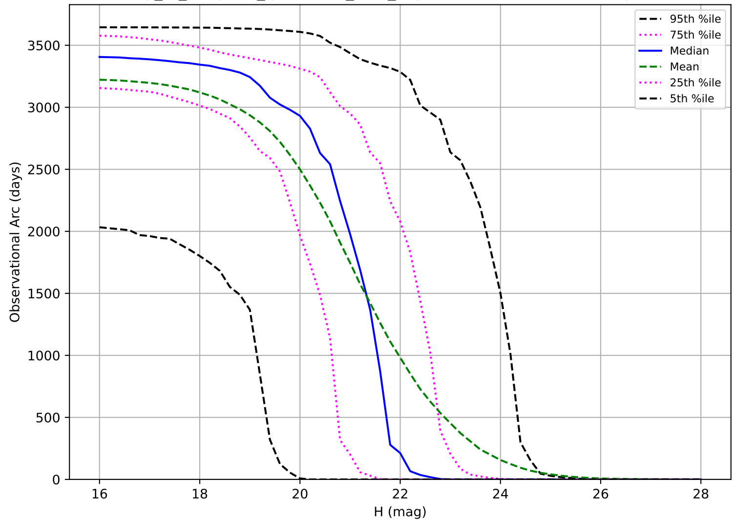
early_ss_template_fpextra2.0_v3.4_10yrs: Observational Arc Length PHA
