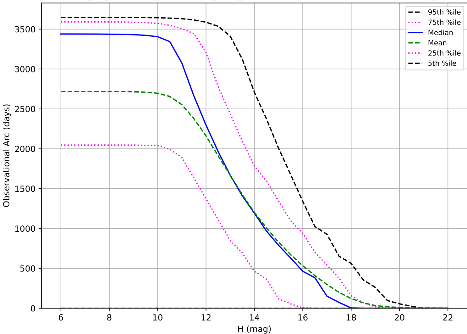
early_ss_template_fpextra2.0_v3.4_10yrs: Observational Arc Length OCC_r5
