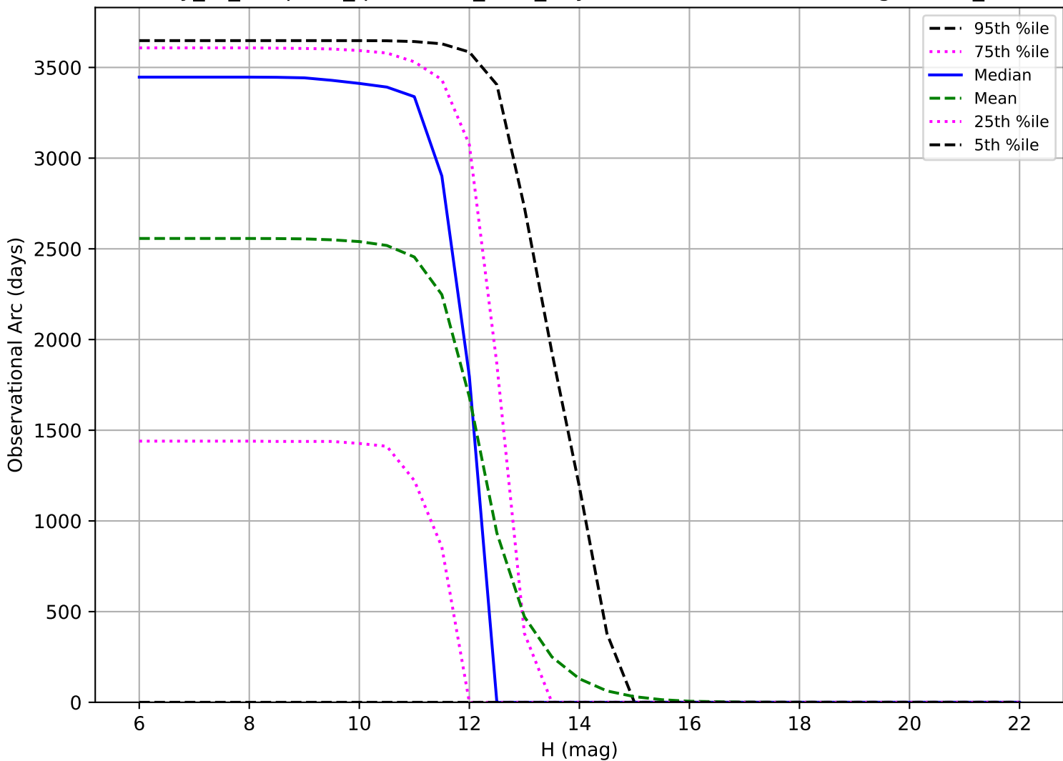
early_ss_template_fpextra2.0_v3.4_10yrs: Observational Arc Length OCC_r20
