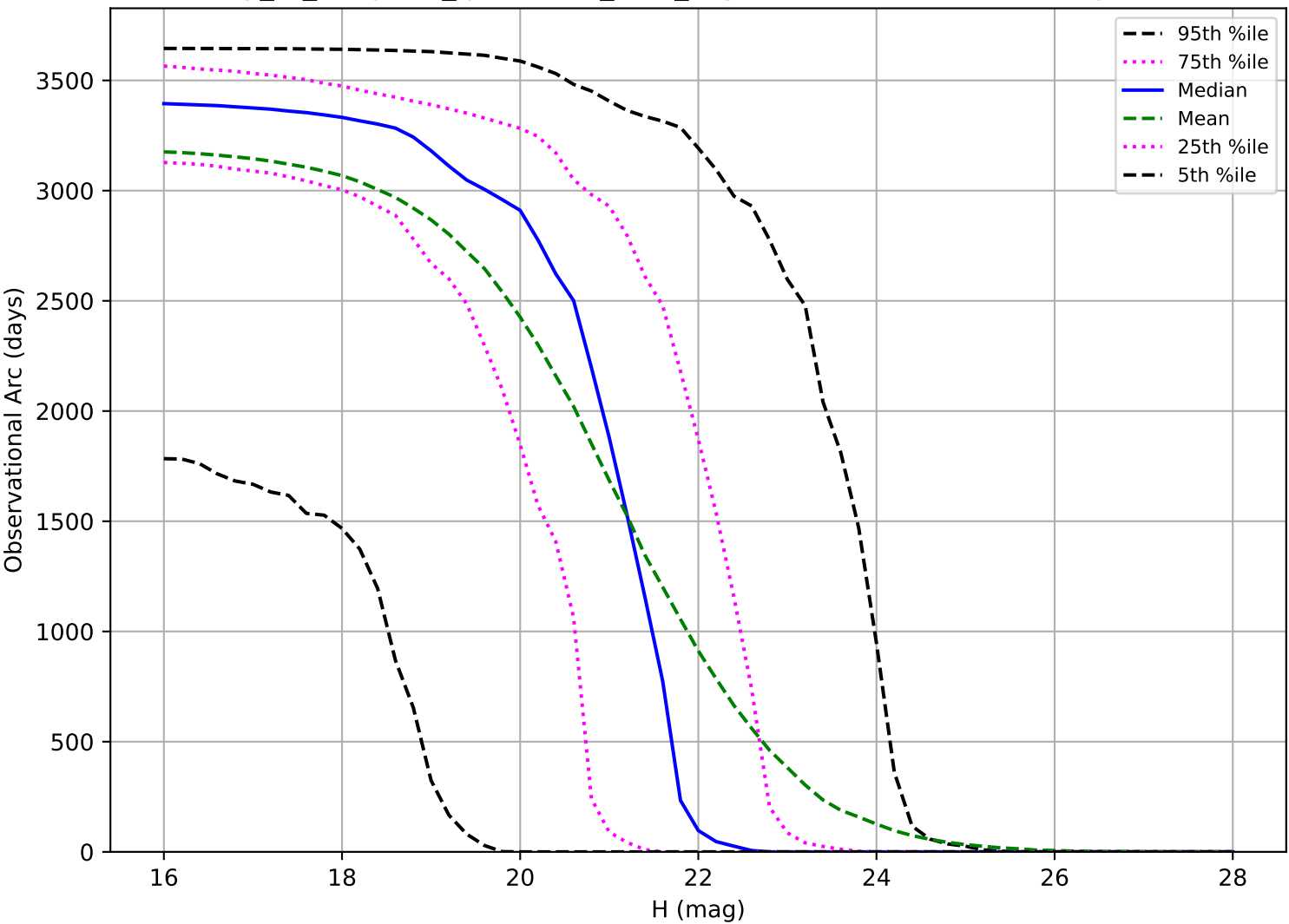
early_ss_template_fpextra2.0_v3.4_10yrs: Observational Arc Length NEO
