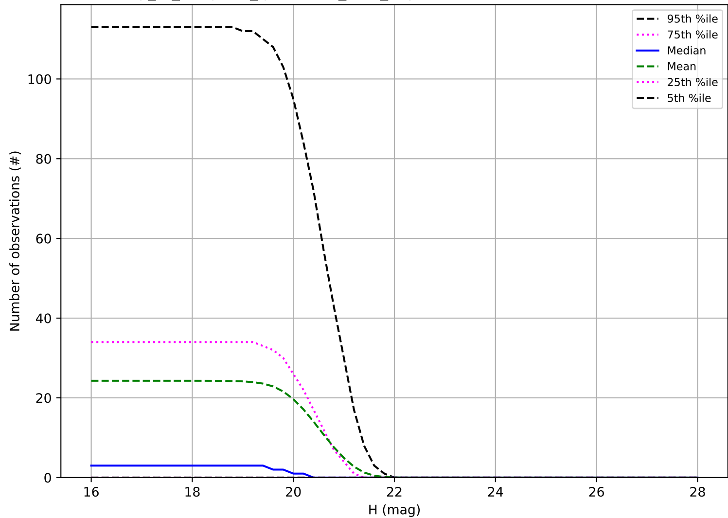
early_ss_template_fpextra2.0_v3.4_10yrs: Number of observations Vatira
