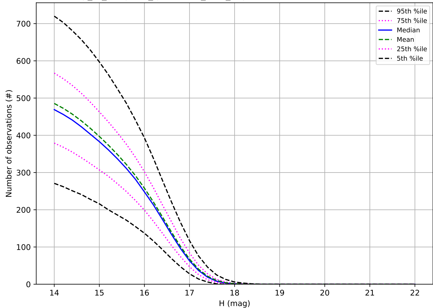
early_ss_template_fpextra2.0_v3.4_10yrs: Number of observations Trojan
