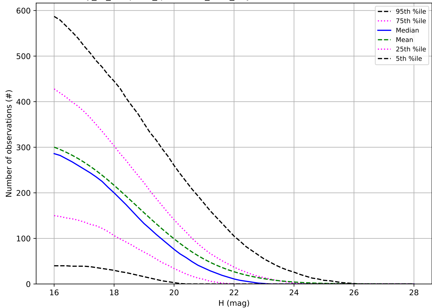
early_ss_template_fpextra2.0_v3.4_10yrs: Number of observations PHA
