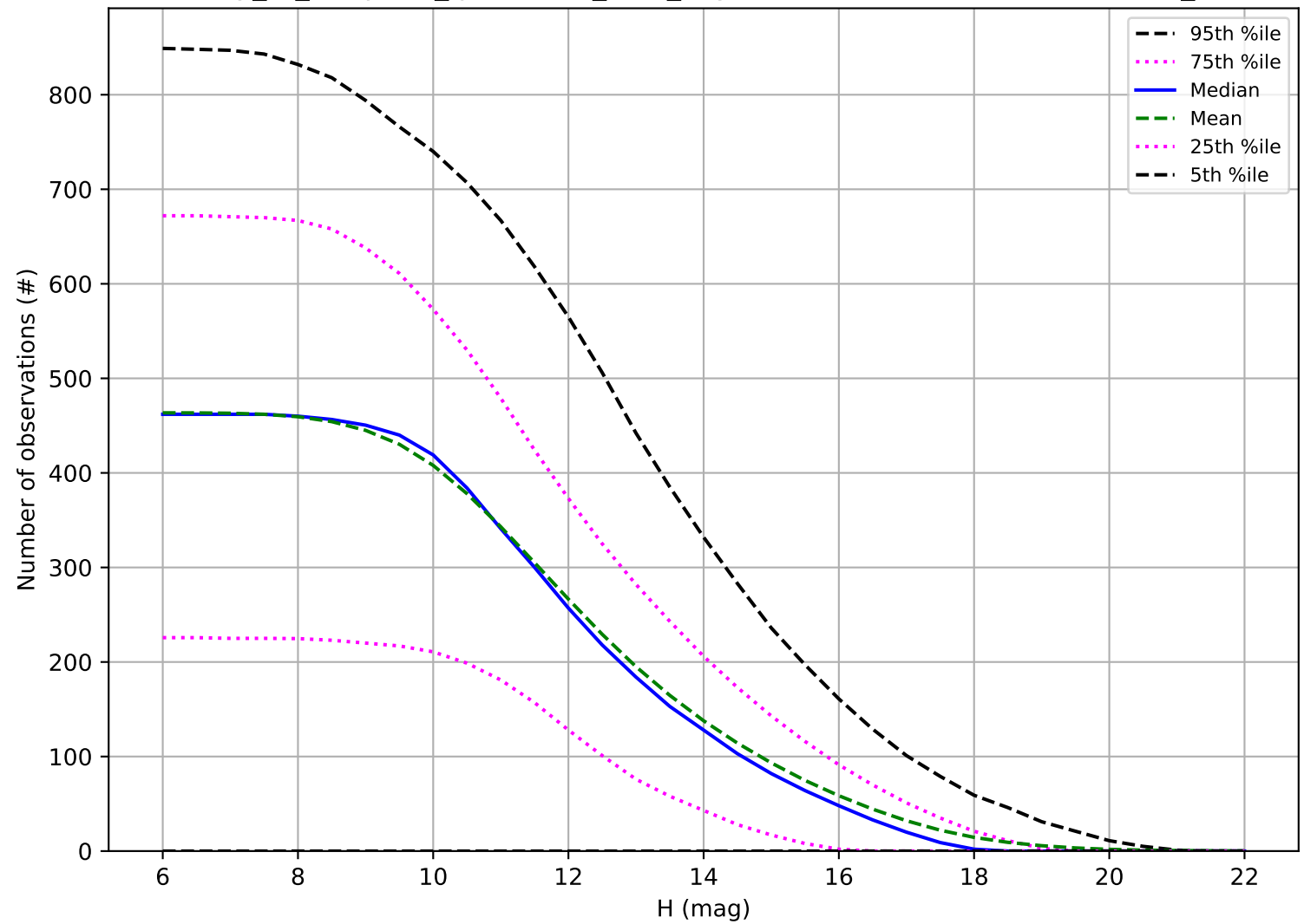
early_ss_template_fpextra2.0_v3.4_10yrs: Number of observations OCC_r5
