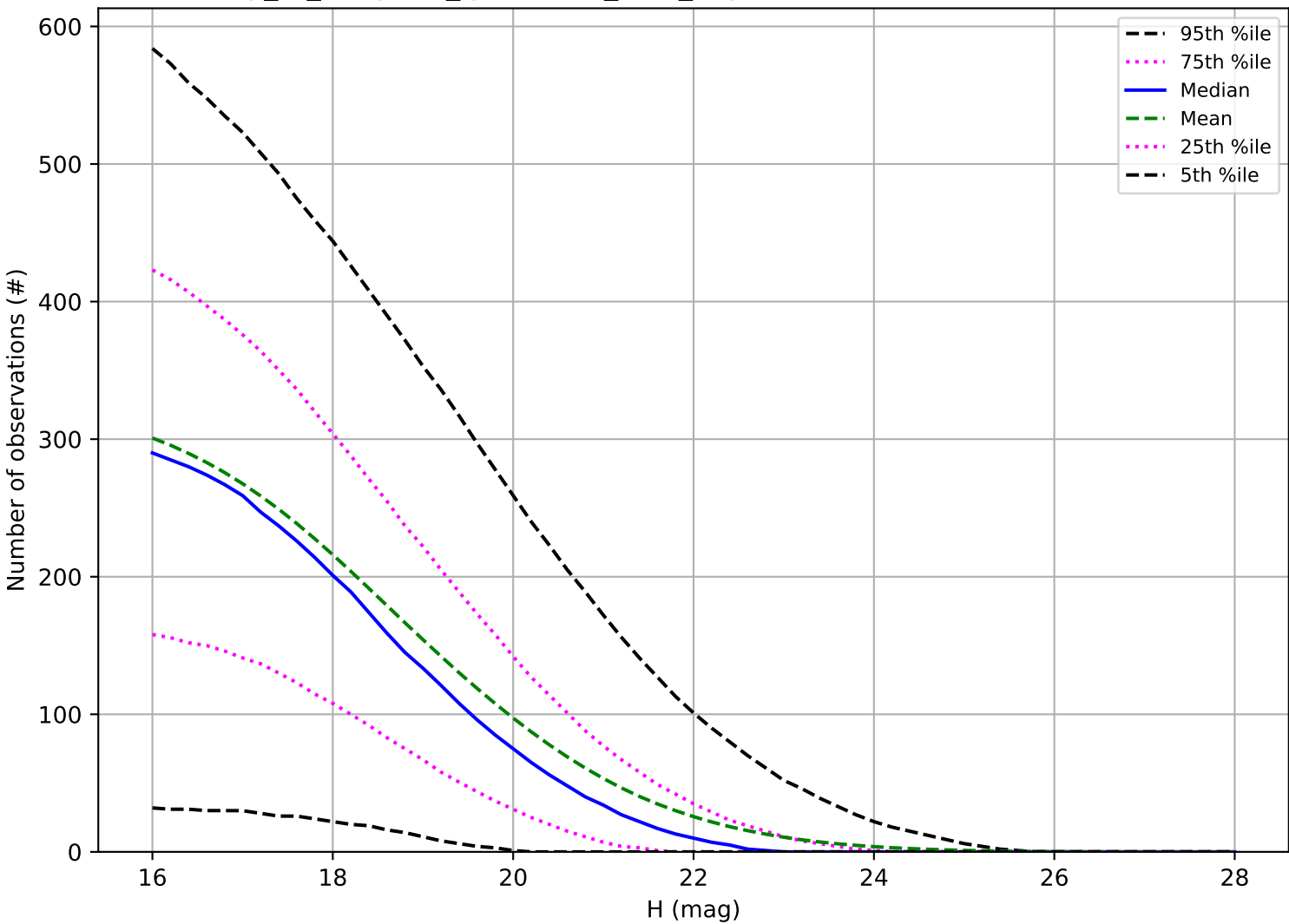
early_ss_template_fpextra2.0_v3.4_10yrs: Number of observations NEO
