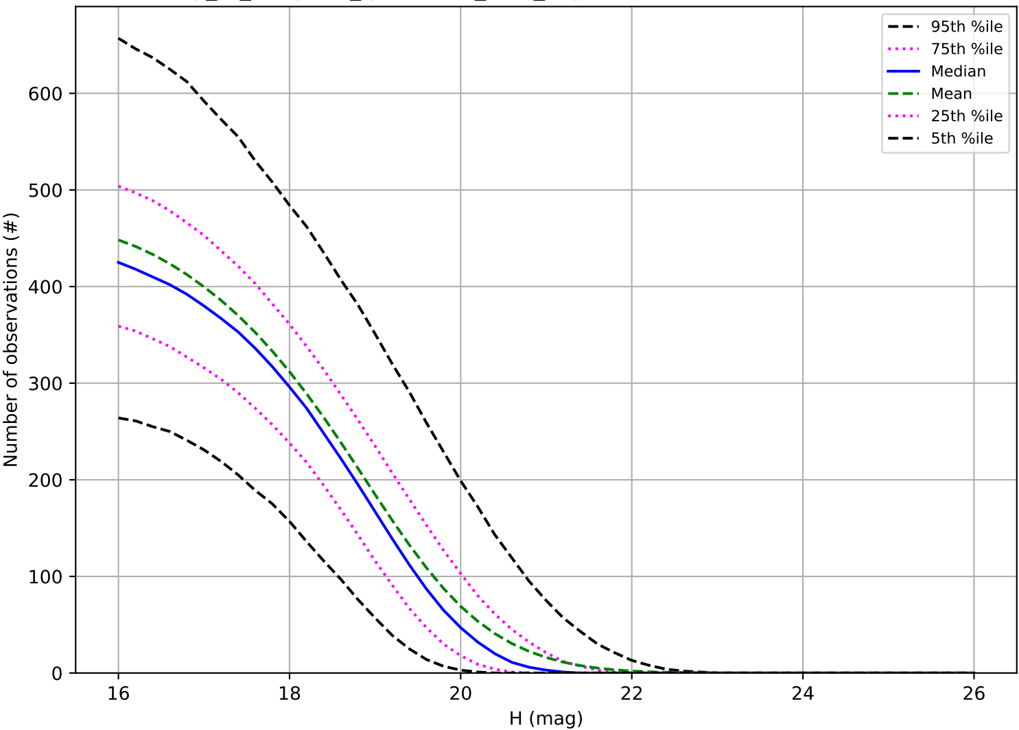
early_ss_template_fpextra2.0_v3.4_10yrs: Number of observations MBA
