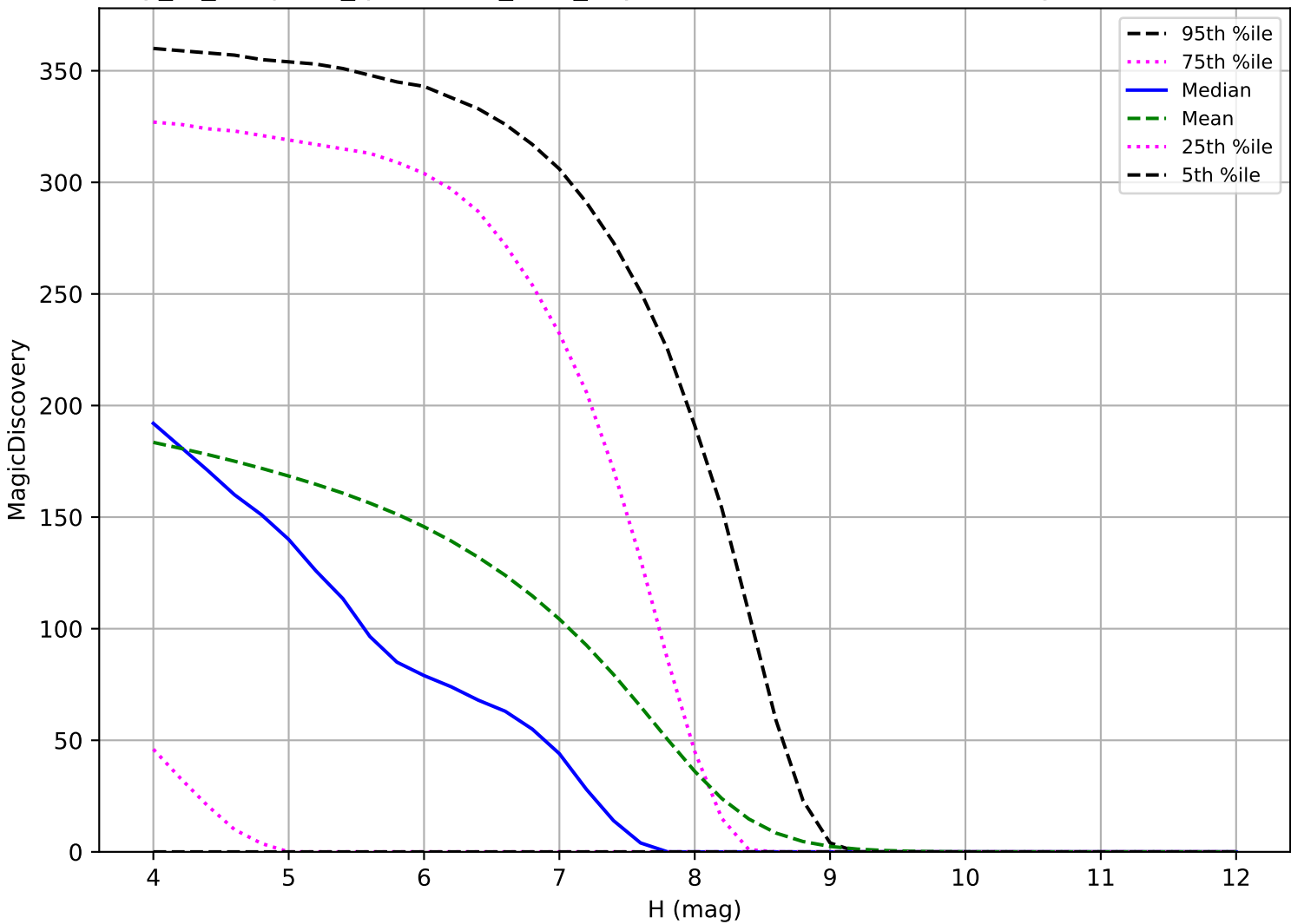
early_ss_template_fpextra2.0_v3.4_10yrs: TNO 6 detections in 60 nights detection loss
