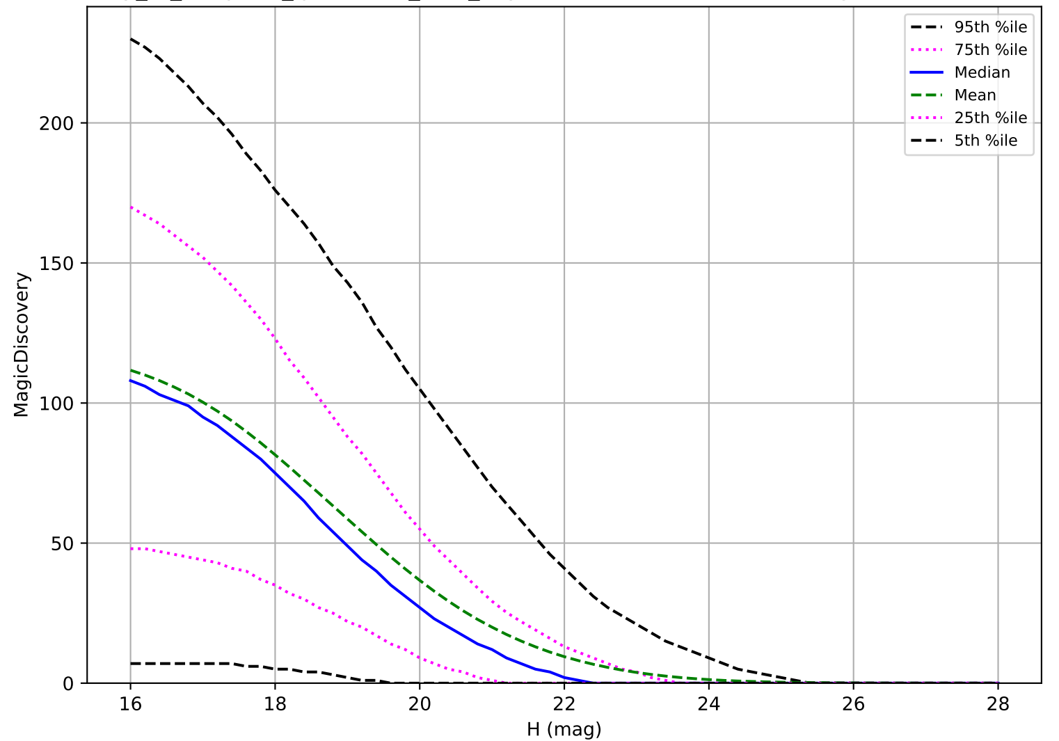
early_ss_template_fpextra2.0_v3.4_10yrs: PHA 6 detections in 60 nights detection loss
