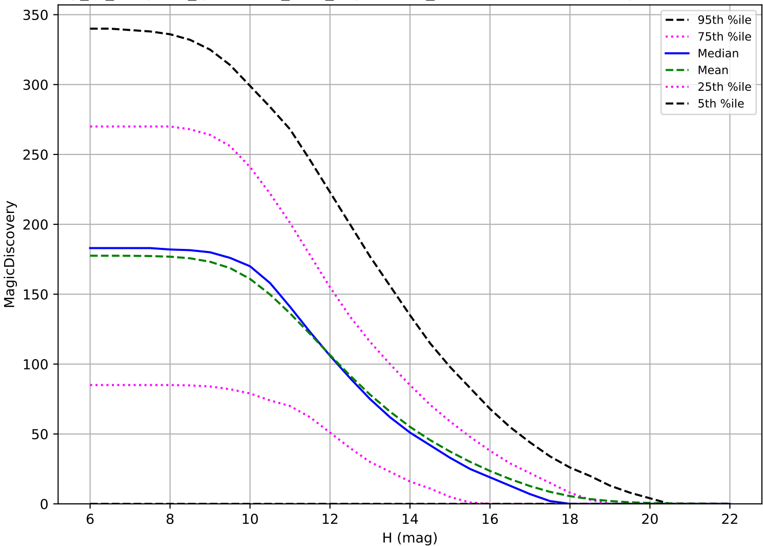
early_ss_template_fpextra2.0_v3.4_10yrs: OCC_r5 6 detections in 60 nights detection loss
