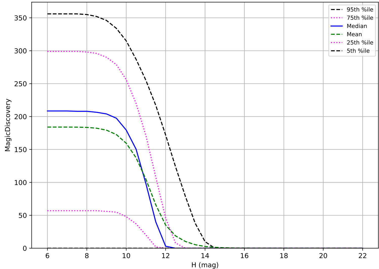
early_ss_template_fpextra2.0_v3.4_10yrs: OCC_r20 6 detections in 60 nights detection loss
