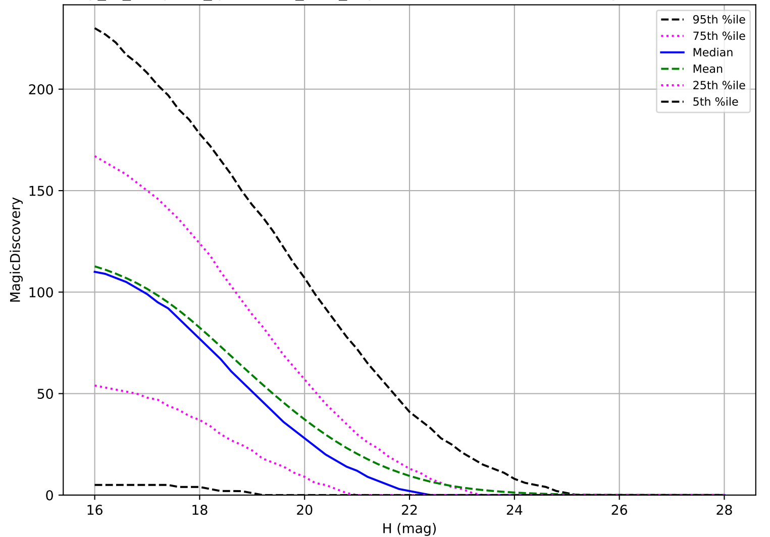
early_ss_template_fpextra2.0_v3.4_10yrs: NEO 6 detections in 60 nights detection loss
