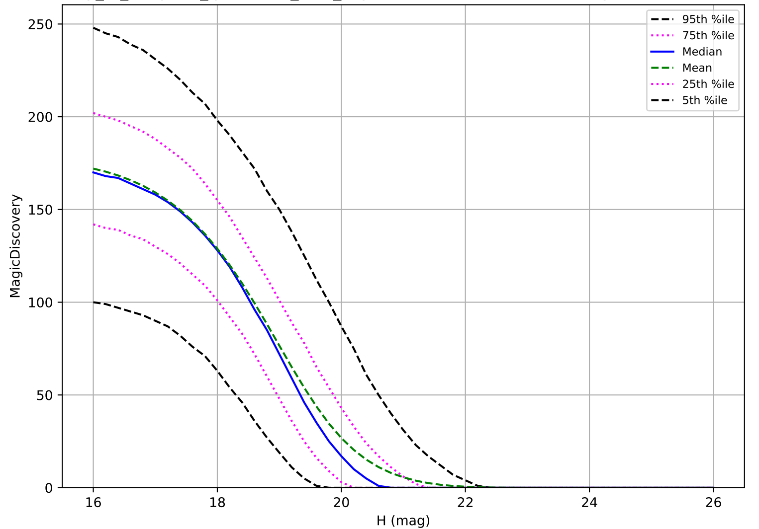
early_ss_template_fpextra2.0_v3.4_10yrs: MBA 6 detections in 60 nights detection loss
